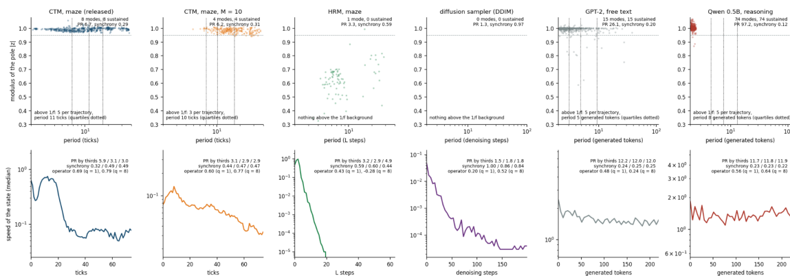
Figure 12: The signature of six networks measured the same way.
