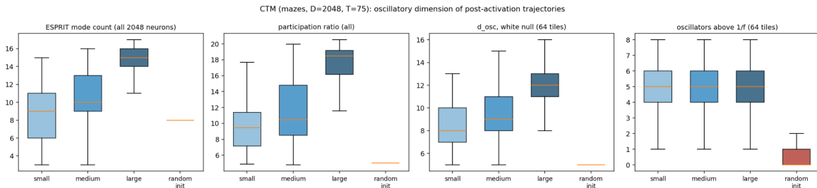
Figure 2: Levels of four estimators in the three maze sets and in the random-weight control.
