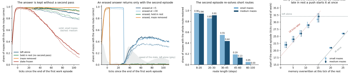
Figure 9: Interventions during the rest of the maze CTM (solid lines: small mazes, dashed: medium).
