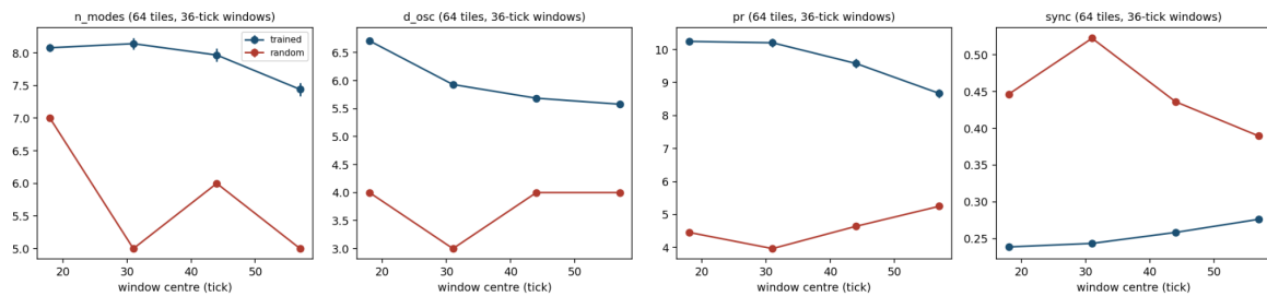
Figure 5: Estimators along internal time for the trained model and the random-weight control (large mazes, 64 tiles).
