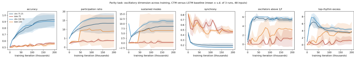
Figure 3: Parity task: accuracy and five dynamical measures across training for CTMs and LSTM baselines with 75 and 100 ticks (mean and standard deviation of three runs).
