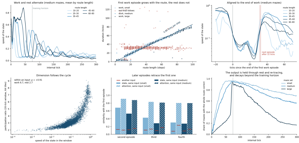
Figure 8: The work–rest cycle of the maze CTM.
