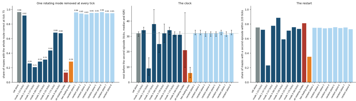
Figure 10: Mode ablation in the released maze CTM. One rotating pair of the operator is removed from the state at every tick (blue; periods in ticks), all rotating pairs with |z| \geq 0.95 together (red), the two leading principal axes (orange) or a random plane (light blue, eight draws).
