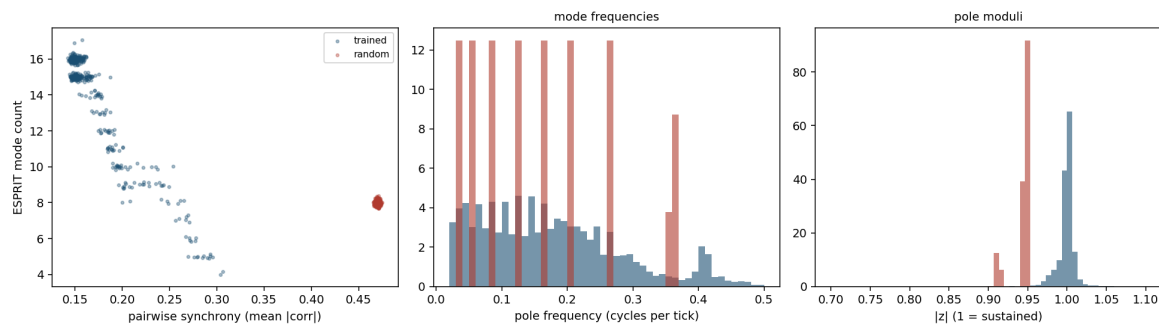
Figure 6: Mode count against pairwise synchrony, and the frequencies and moduli of the ESPRIT poles (trained model and random-weight control).
