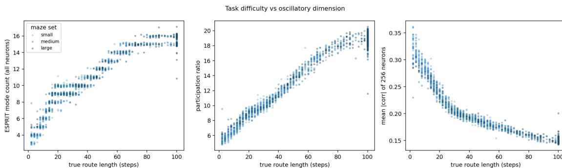
Figure 4: Whole-trajectory mode count, participation ratio and pairwise synchrony against true route length.
