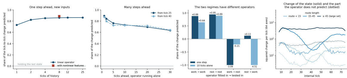
Figure 7: The oscillator operator (maze CTM, 64 principal axes, test inputs).
